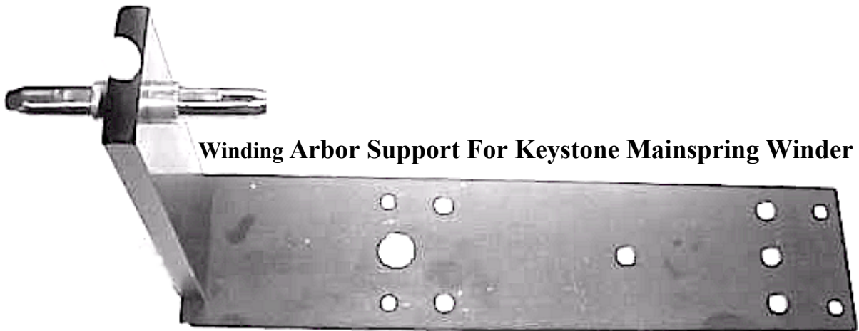
Winding Arbor Support
